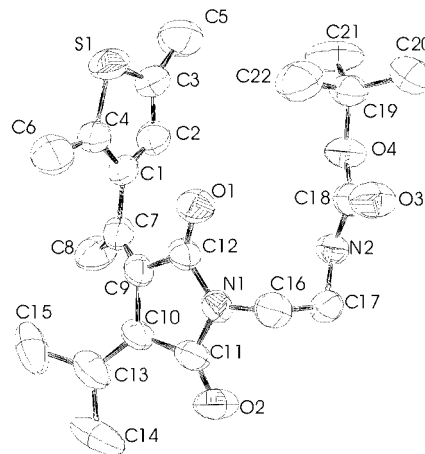
Figure 1. ORTEP plot of ( Z )- 7 ; selected bond lengths [pm], angles [°] and torsion angles [°]: N(1)–C(11) 139.4(6), N(1)–C(12) 139.0(6), C(1)–C(4) 136.7(7), C(1)–C(7) 149.6(6), C(7)–C(9) 133.6(8), C(9)–C(10) 147.0(6), C(10)–C(13) 135.7(7); C(7)–C(9)–C(10) 128.9(5), C(9)–C(10)–C(13) 127.6(5); C(7)–C(9)–C(10)–C(13) –51.0(9), C(12)–C(9)–C(10)–C(11) –17.4(5), C(1)–C(7)–C(9)–C(10) –179.0(5); for further details see Exp. Sect. and ref. [25]
