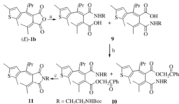
Scheme 3. a) \text{H}_2\text{NCH}_2\text{CH}_2\text{NHBoc} ( 2a ), \text{CH}_2\text{Cl}_2 , reflux, 3 h, quant; b) phenacyl bromide, \text{NEt}_3 , ethyl acetate, room temp., 94%; c) t BuLi (2.4 equiv.), THF, -78^\circ\text{C} , 40%
