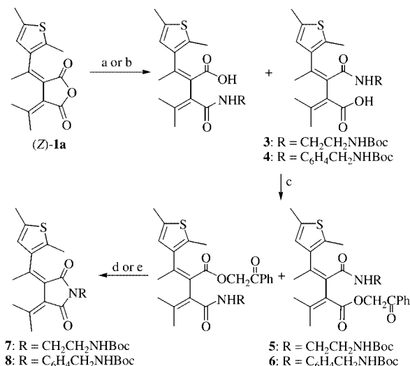
Scheme 2. a) \text{H}_2\text{NCH}_2\text{CH}_2\text{NHBoc} ( 2a ), \text{CH}_2\text{Cl}_2 , reflux, 3 h, 3 : 99%; b) \text{H}_2\text{NC}_6\text{H}_4\text{CH}_2\text{NHBoc} ( 2b ), \text{CH}_2\text{Cl}_2 , reflux, 3 d, 4 : 87%; c) phenacyl bromide, \text{NEt}_3 , ethyl acetate, room temp., 5 : 86%; 6 : 96%; d) Method A: t BuLi (2.2 equiv.), THF, -78^\circ\text{C} , 7 : 48%; 8 : 51% Method B: \text{NEt}_3 (10%), \text{CH}_2\text{Cl}_2 , room temp., 8 : 51%
