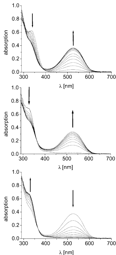
Figure 2. Change of UV/Vis spectra of fulgimide 8 : c = 1.0 \times 10^{-4} mol/L in toluene, XBO 1000 W; top: ( Z )- 8 , 365-nm filter, T_{\text{max}} : 50%, HW: 10 nm, \Delta t = 60 s, pss reached after 600 s; center: ( E )- 8 , 365-nm filter, T_{\text{max}} : 50%, HW: 10 nm, \Delta t = 60 s, pss reached after 540 s; bottom: solution enriched in ( C )- 8 (Entry 4, Table 2, pss 365 ) obtained by irradiation of ( Z )- 8 , 514-nm filter, T_{\text{max}} : 50%, HW: 10 nm, \Delta t = 10 s, pss reached after 80 s
